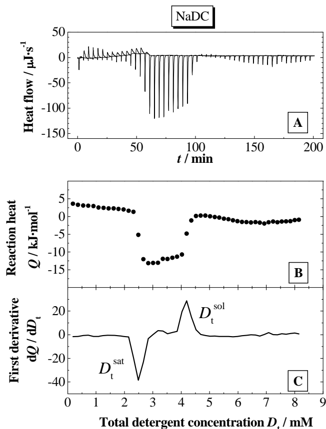
Figure 9. Solubilisation experiment: Titration of a micellar NaDC solution (50 mM) into a DPPC dispersion (6 mM) in 0.1 M NaCl, pH 7.5 at 60 °C with 50 x 5 \mu l. (A) Calorimetric traces, (B) normalised titration heat Q versus total detergent concentration in the cell D_t , (C) first derivative of curve (B).
